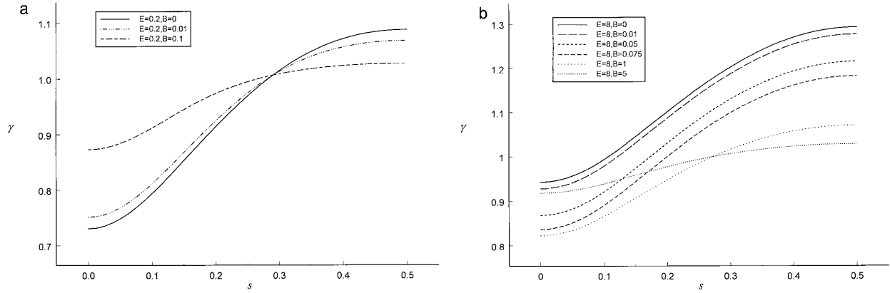
FIG. 17. The surface tension profile \gamma at \text{Ca} = 0.04 for x = 0.5 . All results for \Lambda = 10^3 . (a) E = 0.2 , B = 0 (insoluble), 10^{-2} , and 10^{-1} ; (b) E = 8.0 , B = 0 (insoluble), 10^{-2} , 5 \times 10^{-2} , 7.5 \times 10^{-2} , 1, and 5. Notice that the scales on the figures differ.
