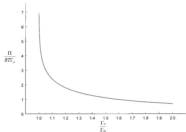
FIG. 2. Surface pressure \pi vs normalized area per molecule \Gamma_\infty/\Gamma_{eq} for the Von Szyckowski model. As the minimum area/molecule is approached, the surface pressure diverges.
