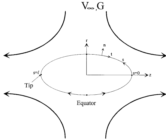
FIG. 1. A neutrally buoyant drop is suspended in an immiscible fluid of equal viscosity and subjected to a pure axisymmetric extensional flow.
