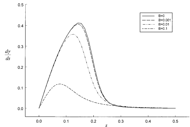
FIG. 5. The Marangoni stress profile at Ca = 0.04 for x = 0.1 . Results are presented for B = 0 (insoluble), 10^{-3} , 10^{-2} , and 0.1 . All results for \Lambda = 10^3 .
