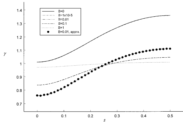
FIG. 9. The surface tension profile \gamma at Ca = 0.04 for x = 0.99 . Results are presented for B = 0 (insoluble), 10^{-5} , 10^{-2} , 0.1 , and 1 . All results for \Lambda = 10^3 . The bold dots indicate results obtained using the approximate mass balance for B = 0.01 , Eq. [33].
