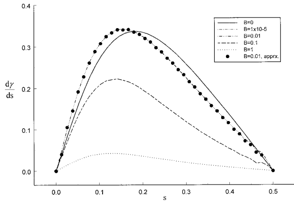
FIG. 10. The Marangoni stress profile at Ca = 0.04 for x = 0.99 . Results are presented for B = 0 (insoluble), 10^{-5} , 10^{-2} , 0.1 , and 1 . All results for \Lambda = 10^3 . The bold dots indicate results obtained using the approximate mass balance for B = 0.01 , Eq. [33].
