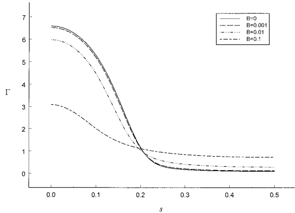
FIG. 3. The surface concentration profile \Gamma at Ca = 0.04 for x = 0.1 . Results are presented for B = 0 (insoluble), 10^{-3} , 10^{-2} , and 0.1 . All results for \Lambda = 10^3 .
