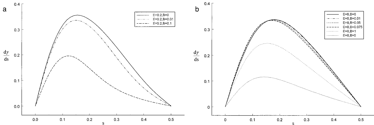
FIG. 18. The Marangoni stress profile at \text{Ca} = 0.04 for x = 0.5 . All results for \Lambda = 10^3 . (a) E = 0.2 , B = 0 (insoluble), 10^{-2} , and 10^{-1} ; (b) E = 8.0 , B = 0 (insoluble), 10^{-2} , 5 \times 10^{-2} , 7.5 \times 10^{-2} , 1, and 5.
