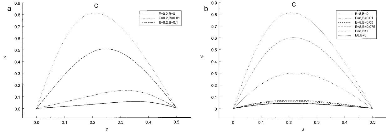
FIG. 19. The tangential surface velocity v_t profile \gamma at Ca = 0.04 for x = 0.5 . All results for \Lambda = 10^3 . (a) E = 0.2 , B = 0 (insoluble), 10^{-2} , and 10^{-1} ; (b) E = 8.0 , B = 0 (insoluble), 10^{-2} , 5 \times 10^{-2} , 7.5 \times 10^{-2} , 1, and 5. Notice that the scales on the figures differ.
