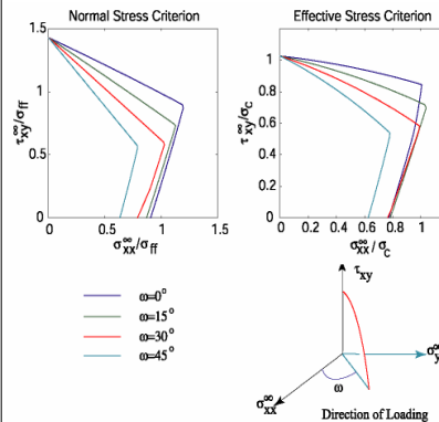
Figure 10: First cracking stress loci. The associated FMC microstructure and micro-constituent properties are related to the geometry and material ratios given in the figure.
