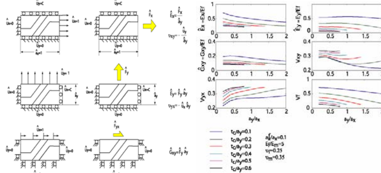
Figure 5: Three boundary value problems simulating the application of stress on a FMC unit cell.
