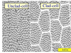
Figure 1: A micrograph showing a FMC microstructure. Several architectures are possible and their effects are investigated elsewhere [1].
