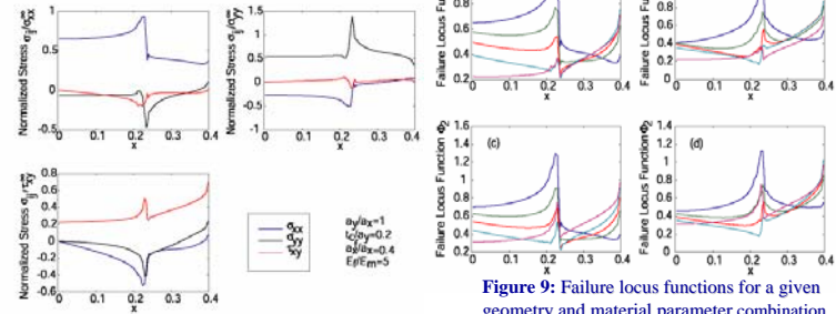
Figure 8: Fundamental micro-stress profiles obtained at the interface between fiber and matrix phases obtained by solving the three independent in-plane boundary value problems.
