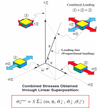
Figure 7: A schematic of a general in-plane loading stress vector.
