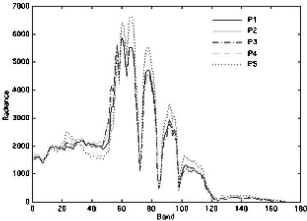
Fig. 7 Spectra of P1, P2, P3, P4, and P5.
